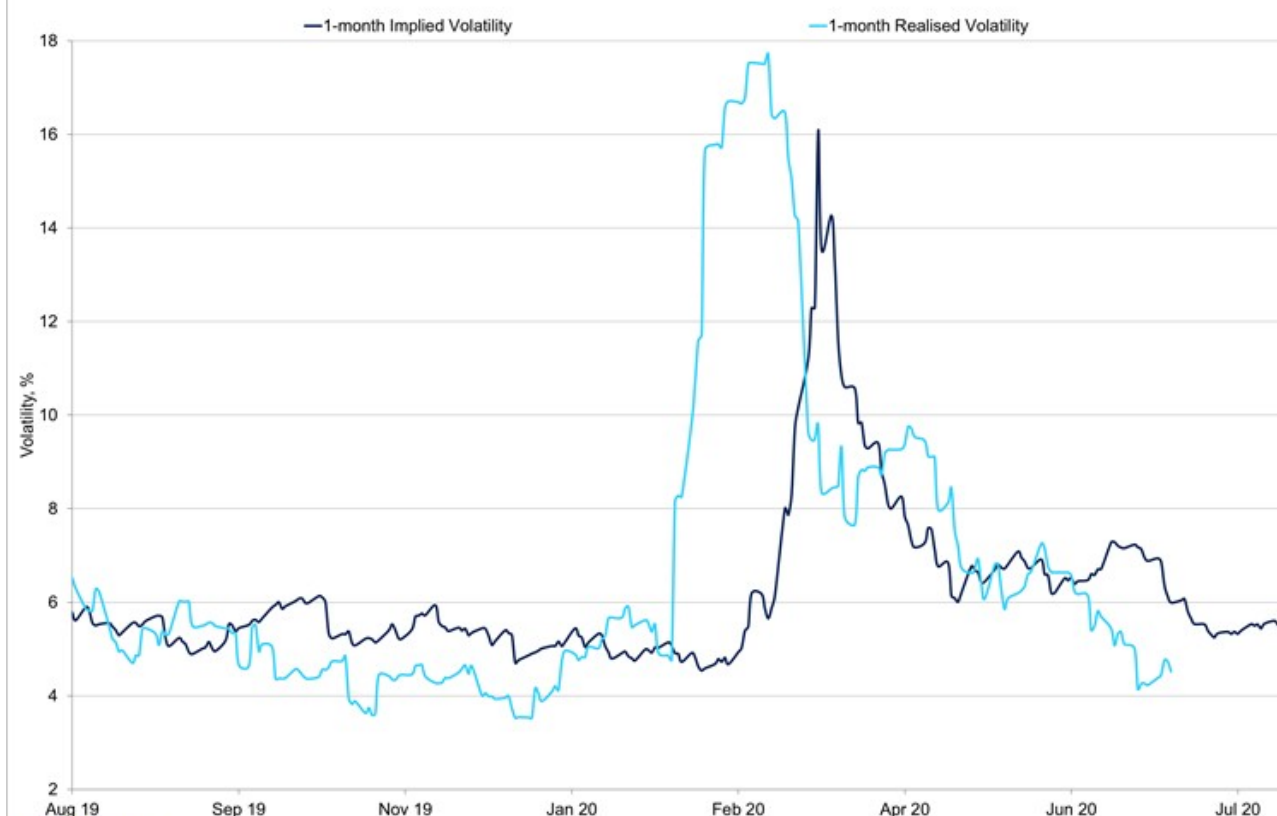
EURSEK 1-month Realised and Implied Volatility
